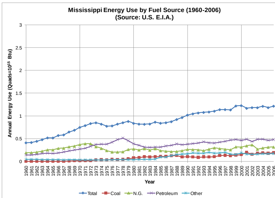
Figure 4.8.3. Mississippi Energy Use by Fuel Source during 1960-2006.
