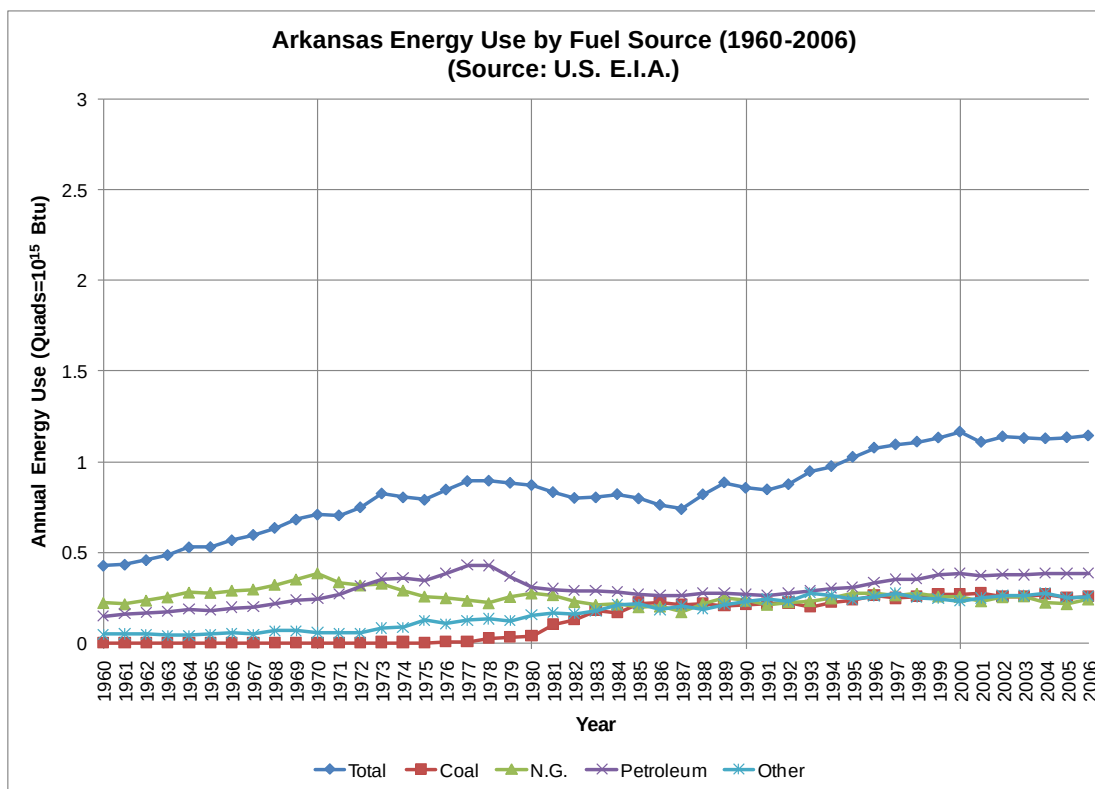
Figure 4.4.3. Arkansas Energy Use by Fuel Source during 1960-2006.
