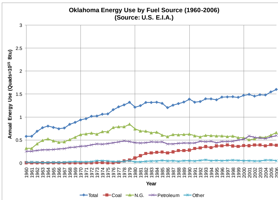
Figure 4.10.3. Oklahoma Energy Use by Fuel Source during 1960-2006.
