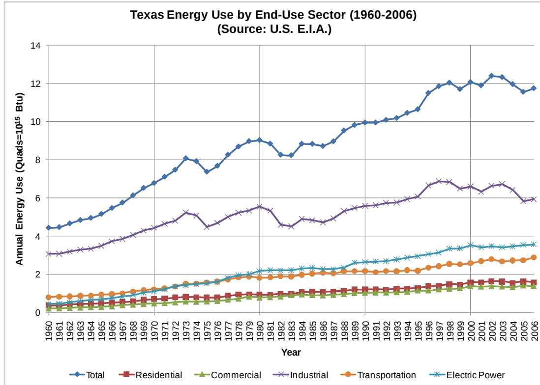
Figure 4.13.1. Texas Energy Use by End-Use Sector during 1960-2006.
