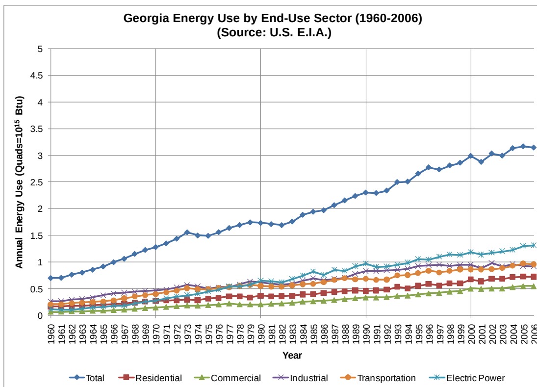
Figure 4.6.1. Georgia Energy Use by End-Use Sector during 1960-2006.
